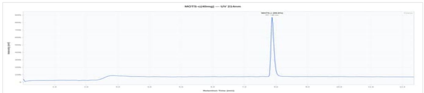
MOTS-C 40mg - AST-MS40-001: UV Chromatogram
