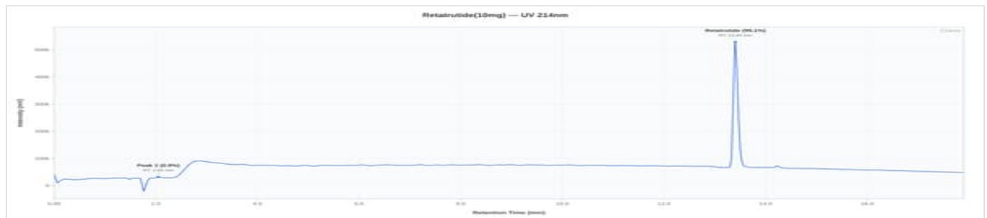
Retatrutide 10mg - AST-RT10-001: UV Chromatogram
