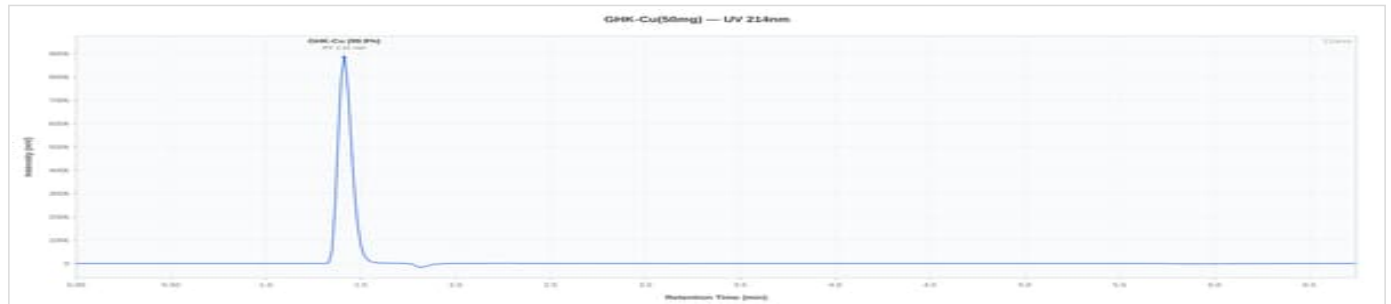
GHK-Cu 50mg - AST-CU-001: UV Chromatogram
